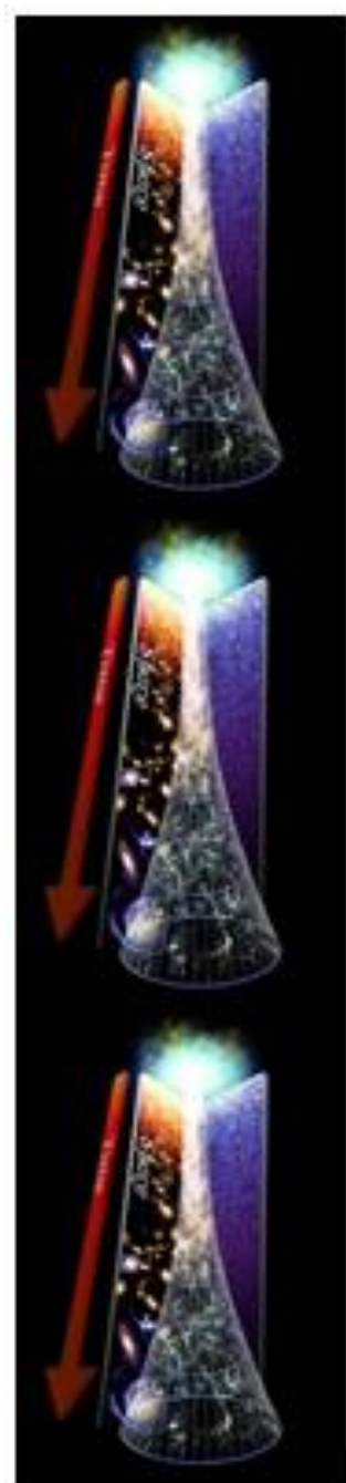
Figure 3: For Mocombe, building on BHBT, the superverses with entangled and superimposed (via black holes) multiverses share the same informational content. So, the hypothesis here is that one superverse created (from the absolute vacuum) a universe, and its informational content is entangled and superimposed on top of another superverse with the informational content of the previous universe emerging in it via black holes. Hence what you have are a layer of multiverses and superverses, superimposed and entangled, whose informational content are shared or recycled via black holes, which organize and structure the multiverses similarly. As such, quantum fluctuation and big bangs are constantly occurring and producing the same worlds, ad infinitum. So, when physicists look out to the cosmic microwave background (CMB), they are looking at the remnant from an early stage of our universe, which came forth from its older version a layer above it, and so on ad infinitum. Put more concretely, the physicists are in a superverse, of our universe, in our milky-way galaxy, looking out to the black hole of a milky-way galaxy from the superverse/multiverse above us with its own consciousness field.
