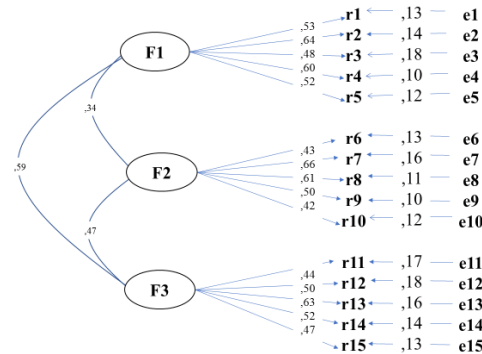
Figure 1: Structural equation modelling
