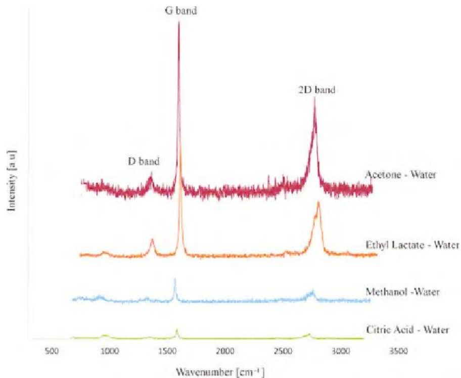
Figure 10: Raman spectra RS of graphene exfoliated via different solvent systems. An increase in the D peak is observed as the lowest R a value of a particular system decreases. This suggests better exfoliation due to the presence of more edges as more layers are exfoliated from bulk- material. It can be seen in Figure that the D band which is associated with edge defects increases gradually when graphene was exfoliated in solvent-water systems that have decreasing Ra- values. This is characteristic of better exfoliation due to formation of the new- edges which leads to a more pronounced edge effect reflected by the increase in the D- peak. From A Facile One-Step Green Synthesis of Graphene by Mild Solvent Exfoliation. Available from: https://www.researchgate.net/publication/303634386_A_Facile_One-Step_Green_Synthesis_of_Graphene_by_Mild_Solvent_Exfoliation [accessed Aug 31 2022]. From A Facile One-Step Green Synthesis of Graphene by Mild Solvent Exfoliation
