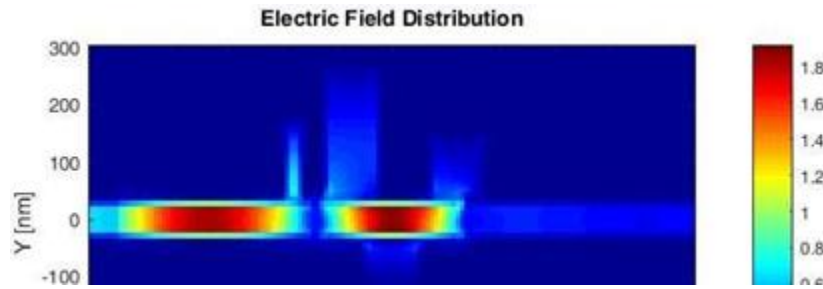
Figure 2: Electric field distribution at resonant frequency
