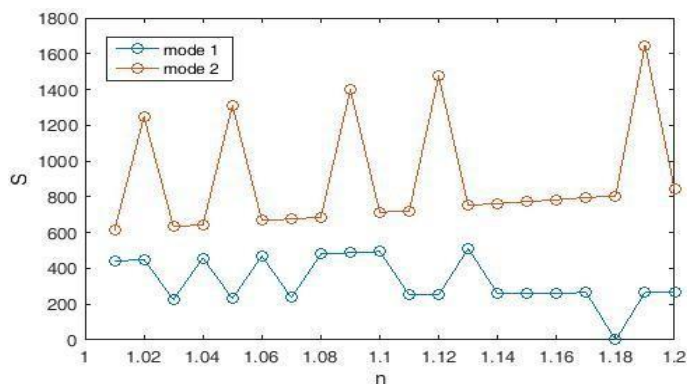
Figure 5: Plasmonic sensor sensitivity coefficient diagram.
